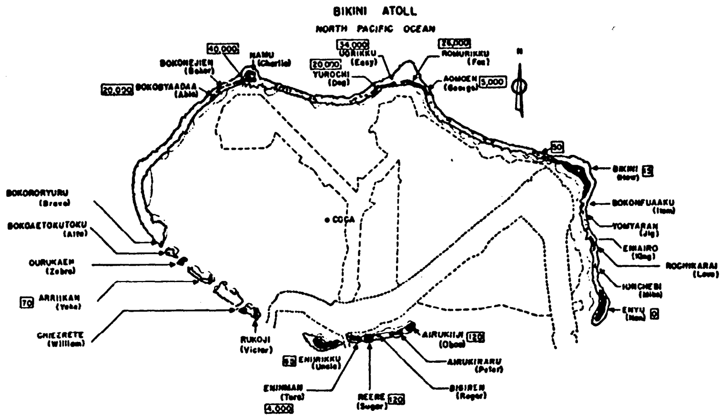
Fig. 3.2 - [Flathead] radiation intensities on Bikini Atoll at H+4 hr, in milliroentgens per hour. Shot site was barge off Yurochi.
