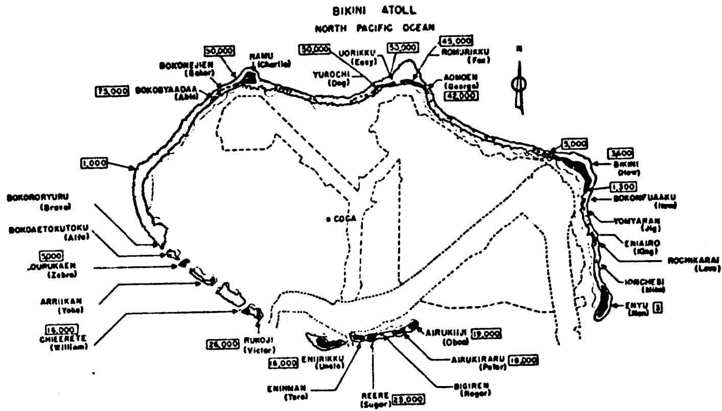
Fig. 3.1 - Zuni Radiation intensities on Bikini Atoll at H+4 hr, in milliroentgens per hour. Shot island was Eninman.
