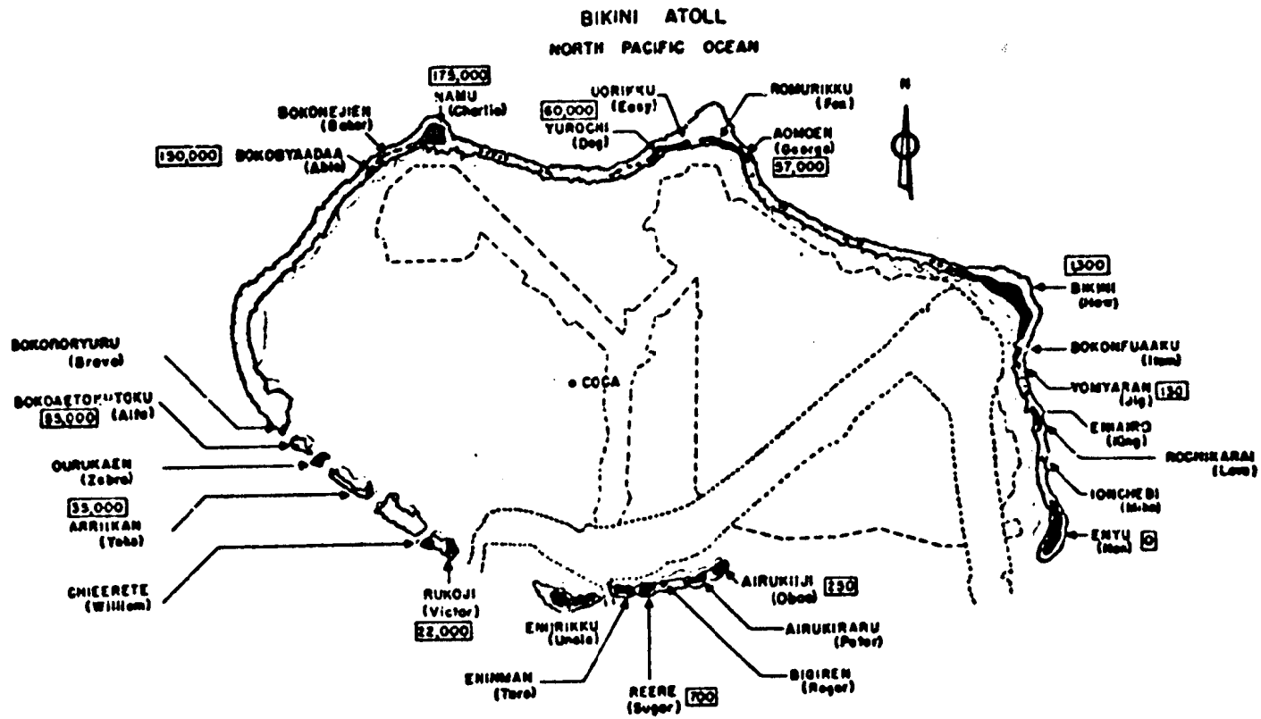
Fig. 3.5- T TEWA radiation intensities on Bikini Atoll at H+4 hr, in milliroentgens per hour. Shot site was barge on reef west of Yurochi.
