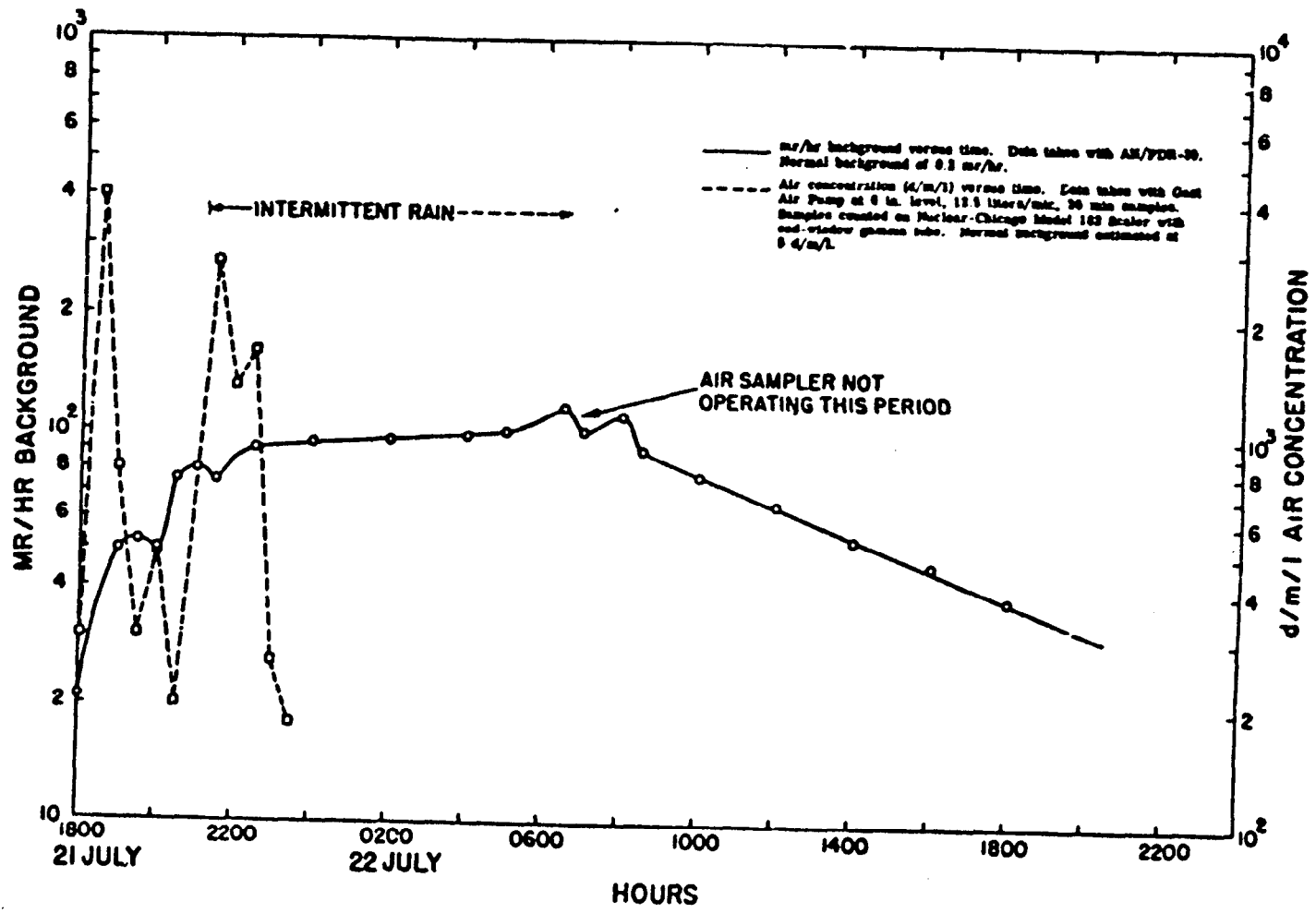
Fig. 2.11—Data on [ TEWA ] fall-out at Rad-Safe Building on Parry Island, Eniwetok Atoll, from 1800 hr, 21 July to 2400 hr, 22 July 1956. Shot was fired at Bikini Atoll.
